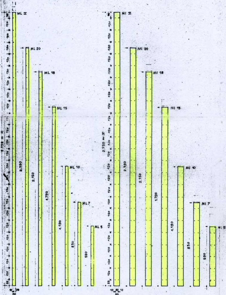
MONTANTS LATéraux CODE: ML PERCEMENTS: TROUS Ø: 5 mm
