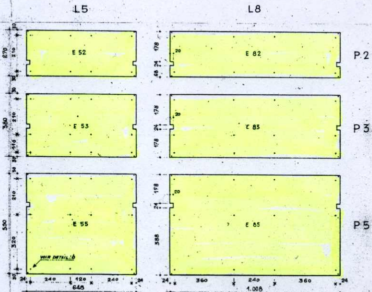
ETAGERES CODE: E PERCEMENTS: TROUS Ø: 5 mm
