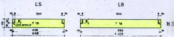
TRAVERSES CODE: T PERCEMENTS: DETAIL: C
